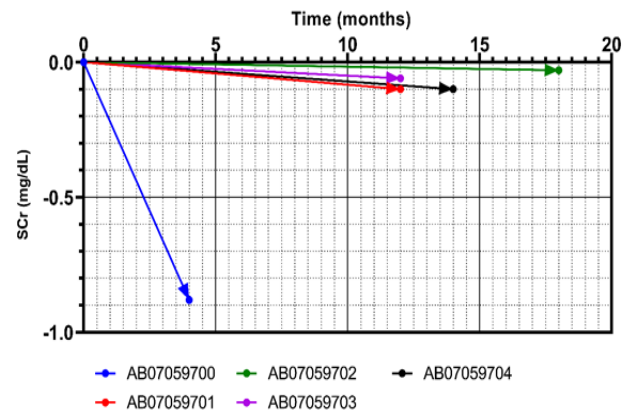
FIGURE 3: SCr a : Change from Treatment-Baseline Vectors
